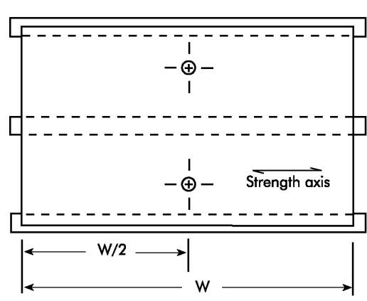
Figure 4. Uniform Load Test Specimen Diagram shows strength axis parallel to supports.
