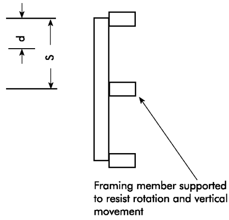
Figure 4. Uniform Load Test Specimen Diagram shows strength axis parallel to supports.
